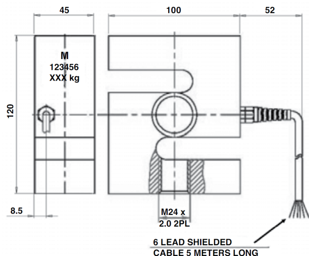
3000, 5000 kg cell outline
